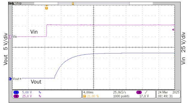
4.00 ms/div rMOR2812S start-up response FIGURE 45
