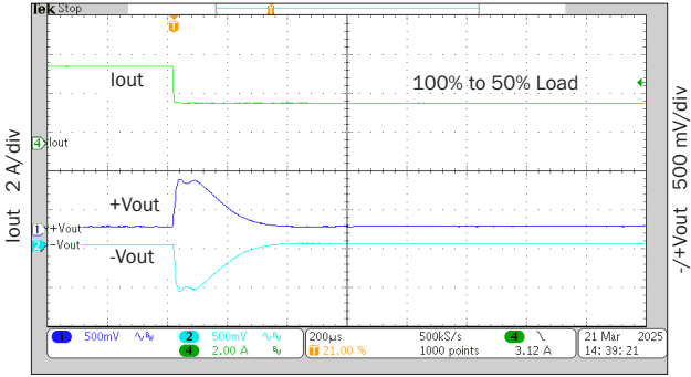
200 μs/div rMOR2815D step load response FIGURE 85
