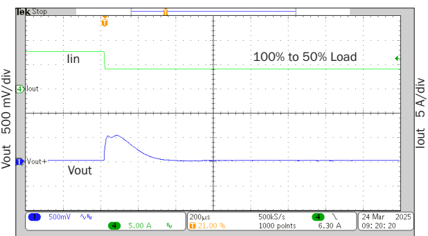
200 μs/div rMOR2815S step load response FIGURE 55
