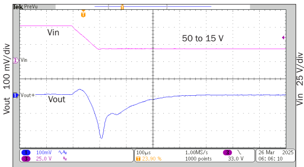
100 μs/div rMOR2815S step line response FIGURE 53
