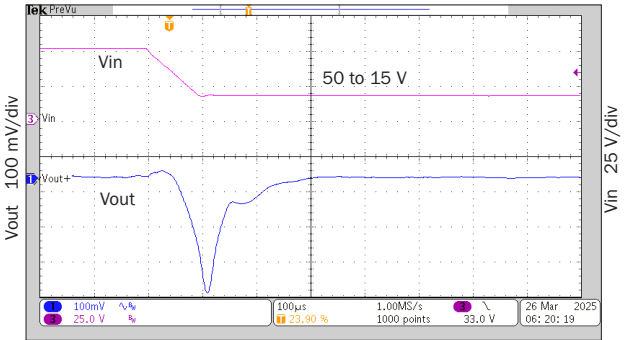
100 \mu s/div rMOR289R5S step line response FIGURE 41
