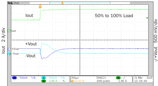
200 μs/div rMOR2812D step load response
