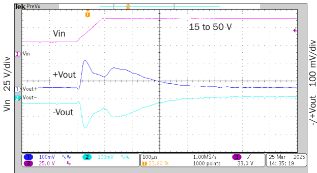
100 μs/div rMOR2812D step line response
