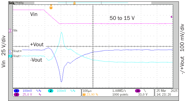
100 μs/div rMOR2815D step line response FIGURE 83
