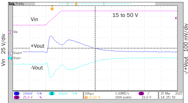
100 μs/div rMOR2815D step line response FIGURE 82
