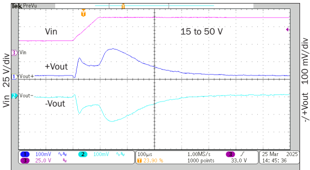
100 \mu s/div rMOR289R5D step line response
