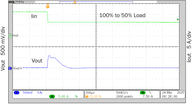
200 \mu s/div rMOR289R5S step load response FIGURE 43
