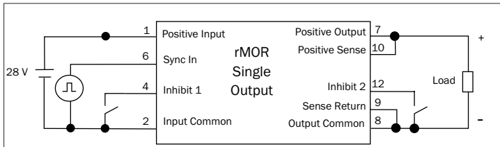
FIGURE 10: TYPICAL CONNECTIONS WITH SENSE PIN
