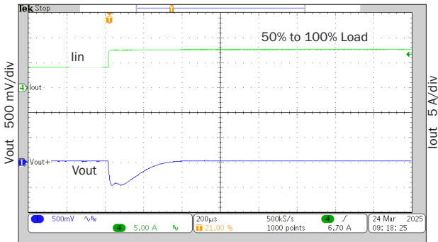
200 μs/div rMOR2815S step load response FIGURE 54
