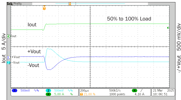
200 \mu s/div rMOR289R5D step load response
