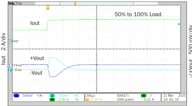
200 μs/div rMOR2815D step load response FIGURE 84
