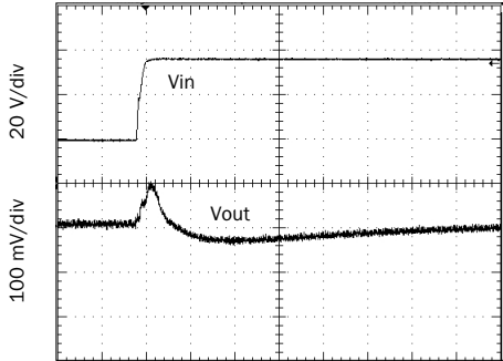
Vin 19 TO 56 V, full resistive load SMRT2805S Representative of Single Output Line Transient FIGURE 21
