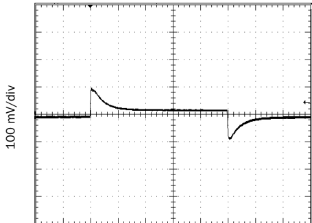
Load 50 - 100 - 50%, 28 Vin SMRT2805S Representative of Single Output Load Transient FIGURE 23
