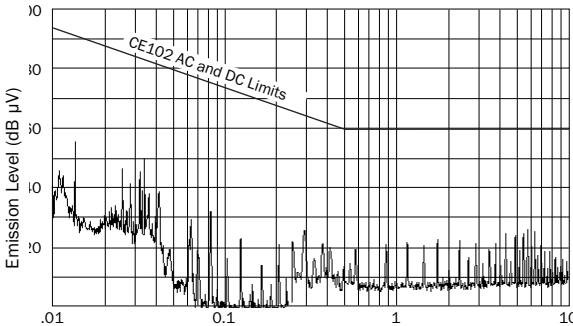
Frequency (MHz), 28 V_{IN} SMRT Single MIL-STD-461 D-F, CE102 FIGURE 19
