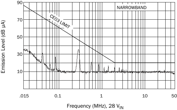
SMRT Dual MIL-STD-461C, CE03
