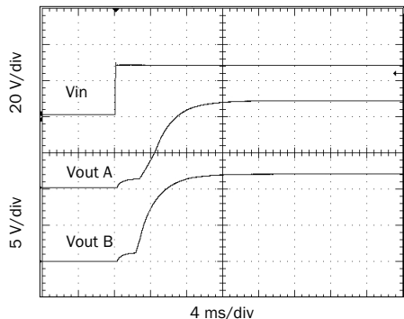
Full resistive load, 28 Vin SMRT2812D Representative of Dual Turn On Delay FIGURE 41
