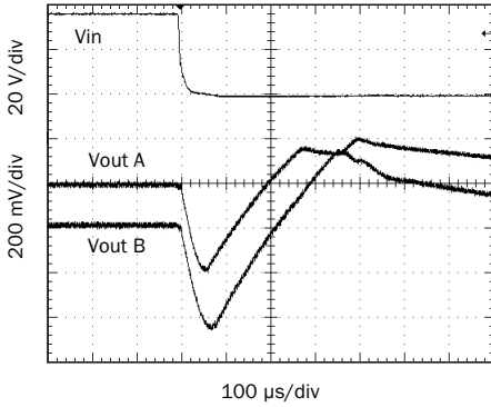
Vin 56 to 19 V, full resistive load SMRT2812D Representative of Dual Output Line Transient FIGURE 38
