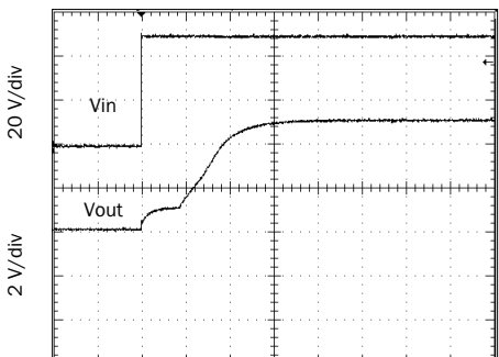
Full resistive load, 50 Vin SMRT2805S Representative of Single Turn On Delay FIGURE 26
