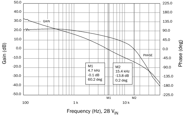
SMRT2815D Gain Phase FIGURE 32
