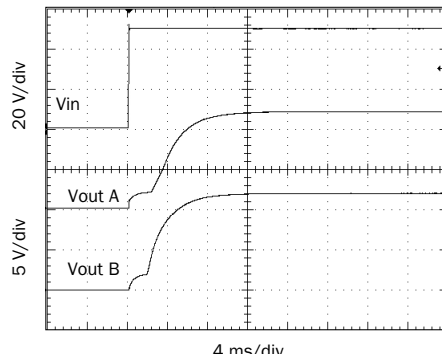
Full resistive load, 50 Vin SMRT2812D Representative of Dual Turn On Delay FIGURE 42
