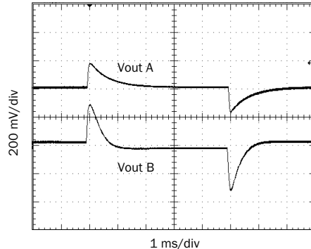
Load 50 - 100 - 50%, 50 Vin SMRT2812D Representative of Dual Output Load Transient FIGURE 40
