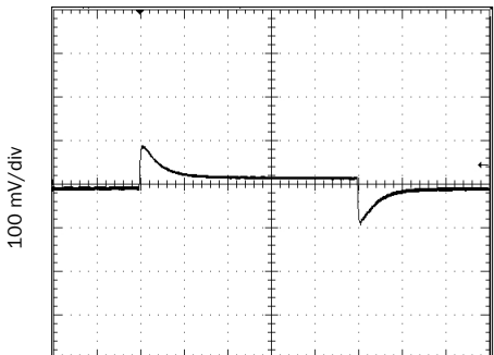
Load 50 - 100 - 50%, 50 Vin SMRT2805S Representative of Single Output Load Transient FIGURE 24
