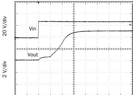
Full resistive load, 28 Vin SMRT2805S Representative of Single Turn On Delay FIGURE 25
