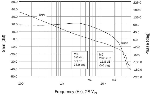
SMRT2805D Gain Phase FIGURE 28
