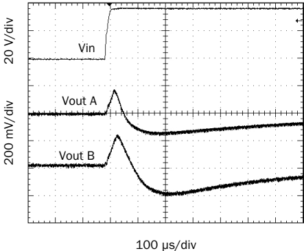
Vin 19 to 56 V, full resistive load SMRT2812D Representative of Dual Output Line Transient FIGURE 37
