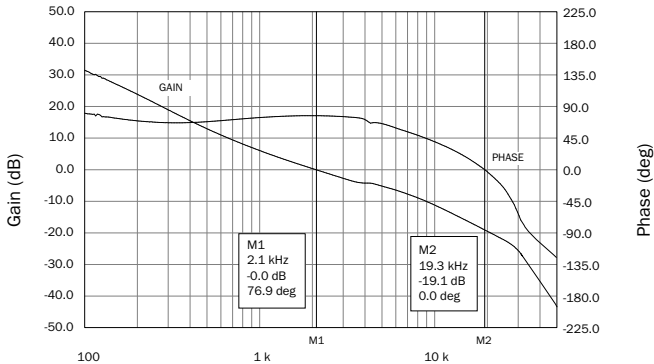
Frequency (Hz), 28 V_{IN} SMRT28507T Gain Phase, +Aux FIGURE 48
