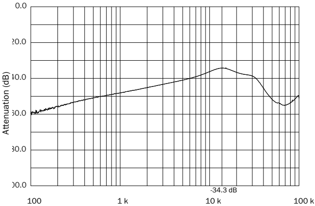
Frequency (Hz), 28 V_{IN} SMRT Single Audio Rejection FIGURE 20
