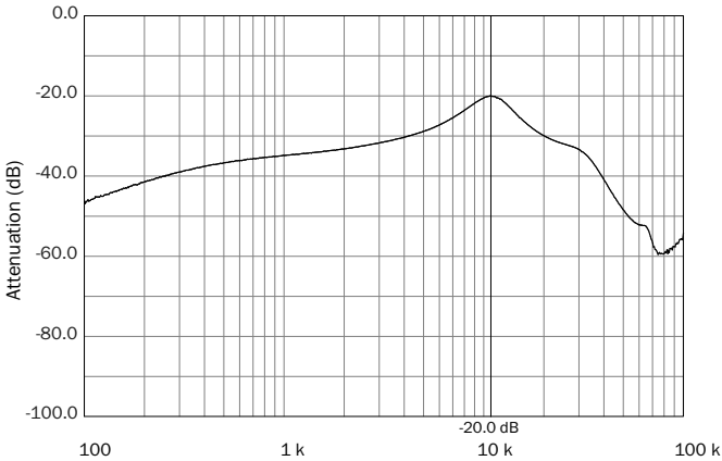
SMRT Dual Audio Rejection, Vout A
