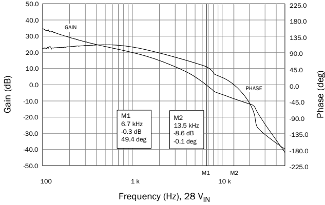
SMRT2812D Gain Phase FIGURE 30
