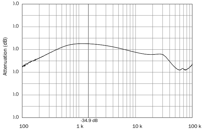
SMRT Triple Audio Rejection, +Aux FIGURE 56
