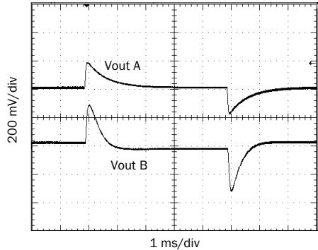
Load 50 - 100 - 50%, 28 Vin SMRT2812D Representative of Dual Output Load Transient FIGURE 39
