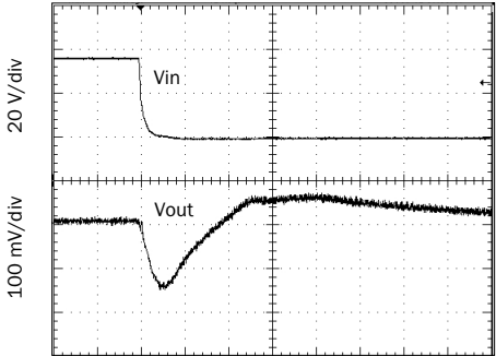
Vin 56 TO 19 V, full resistive load SMRT2805S Representative of Single Output Line Transient FIGURE 22
