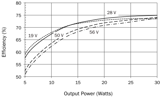
SMRT28512T Efficiency FIGURE 49
