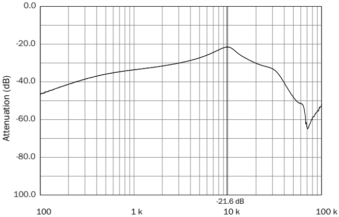
SMRT Dual Audio Rejection, Vout B
