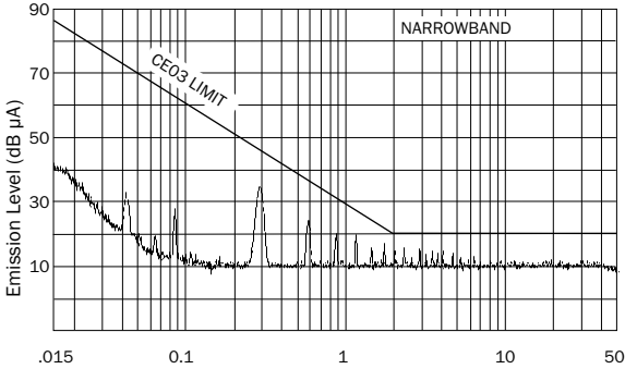
Frequency (MHz), 28 V_{IN} SMRT Single MIL-STD-461C, CE03 FIGURE 18
