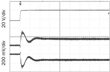
100 µs/div Vin 16 to 40 to 16 Volts, full resistive load Representative of Dual Output Line Transient
