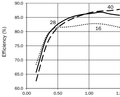
Output Power (Watts) SLH2815D Efficiency
