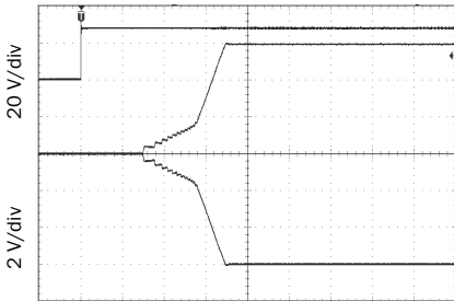
Representative of Dual Output Turn-On Delay
