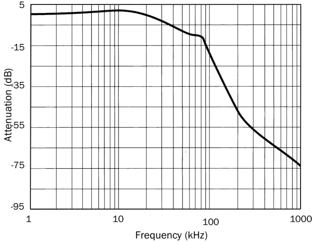
SFMC28-461 Typical Amplitude Response vs. Frequency
