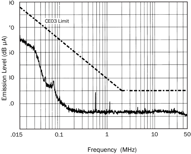
DC-DC Converter Typical EMI With SFMC28-461 Filter
