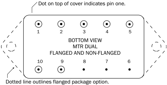
Dotted line outlines flanged package option. See Figure 33 on page 21, Figure 34 on page 22, Figure 36 on page 24 and Figure 37 on page 25 for dimensions.
