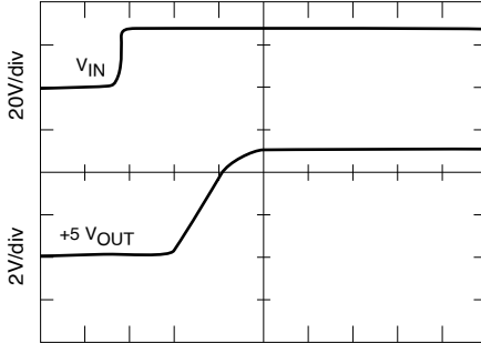
500 µs/div MTR28515T, MAIN (+5) TURN-ON INTO FULL LOAD
