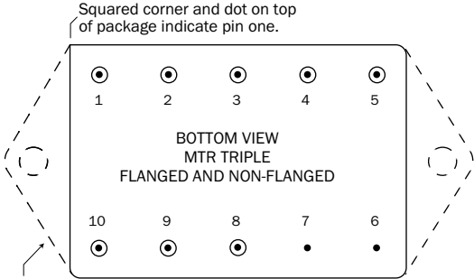
Dotted line outlines flanged package option. See Figure 32 on page 20 and Figure 35 on page 23 for dimensions.
