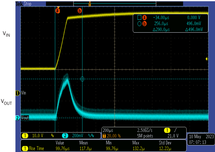
UNITS ARE PER DIVISION MSA+2805S STEP LINE 15 - 50 VOLTS FULL LOAD
