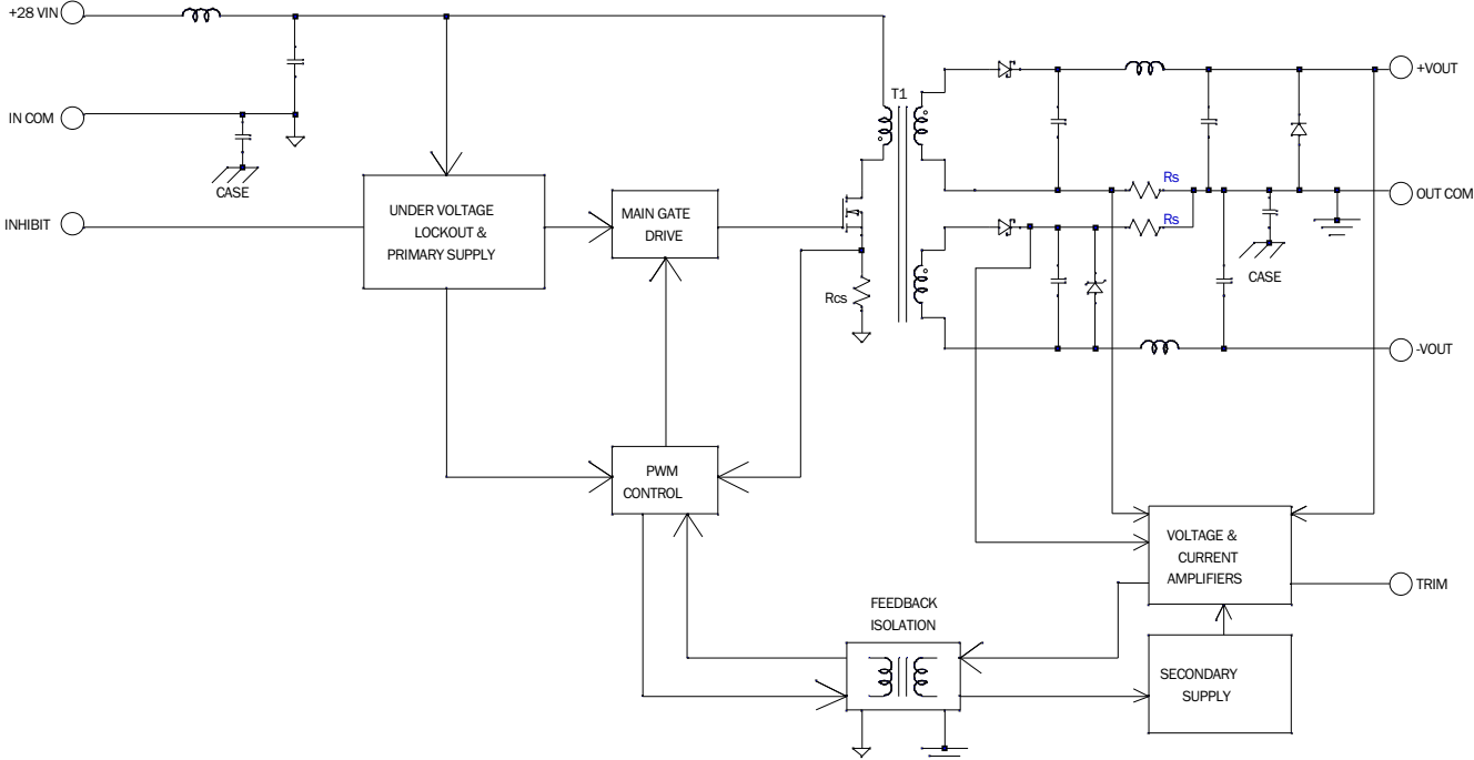
FIGURE 4: BLOCK DIAGRAM MSA+ DUAL OUTPUT
