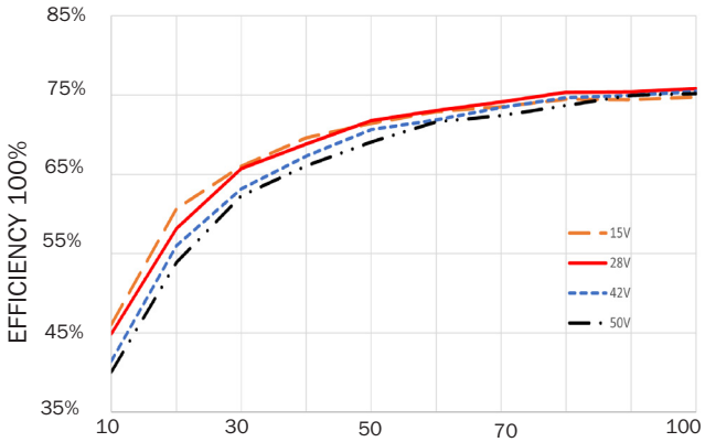
OUTPUT POWER MSA+2805D EFFICIENCY FIGURE 21
