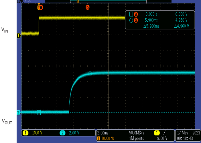
UNITS ARE PER DIVISION MSA+2805D START-UP RESPONSE FULL LOAD FIGURE 32
