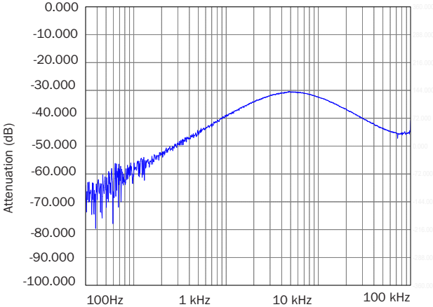
MSA+2805S SINGLE AUDIO REJECTION FIGURE 12
