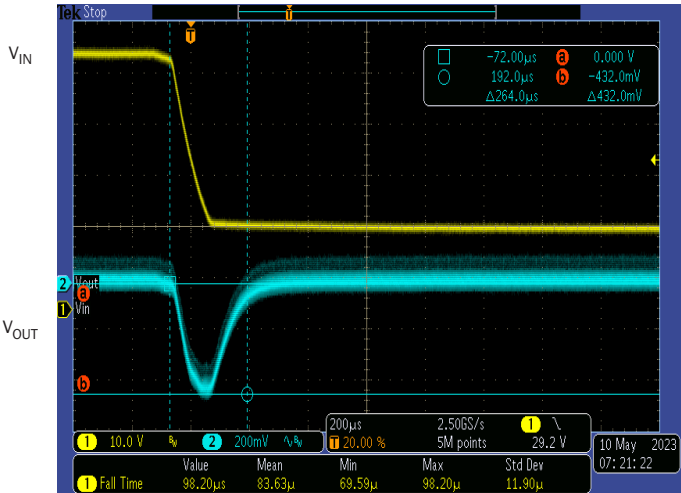
UNITS ARE PER DIVISION MSA+2805S STEP LINE 50 - 15 VOLTS FULL LOAD
