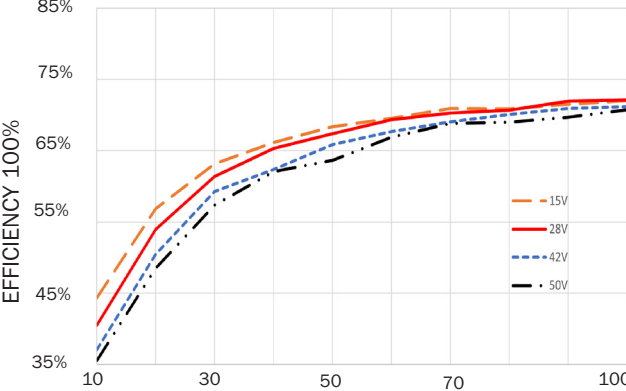
OUTPUT POWER MSA+28R3RS EFFICIENCY FIGURE 7
