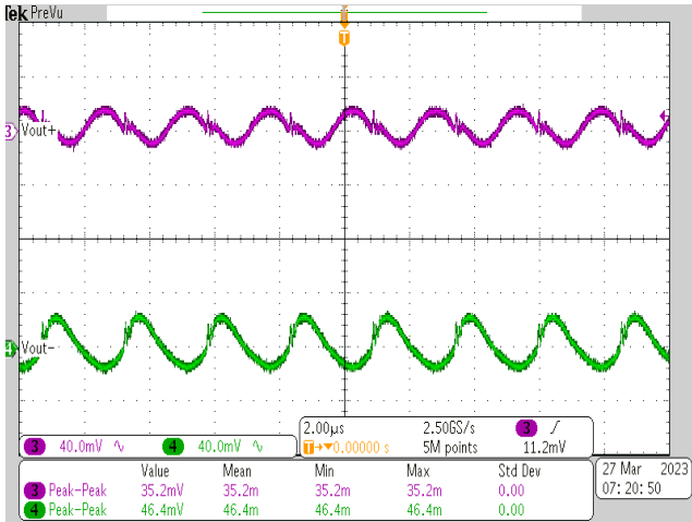
UNITS ARE PER DIVISION MSA+2805D OUTPUT RIPPLE FIGURE 26
