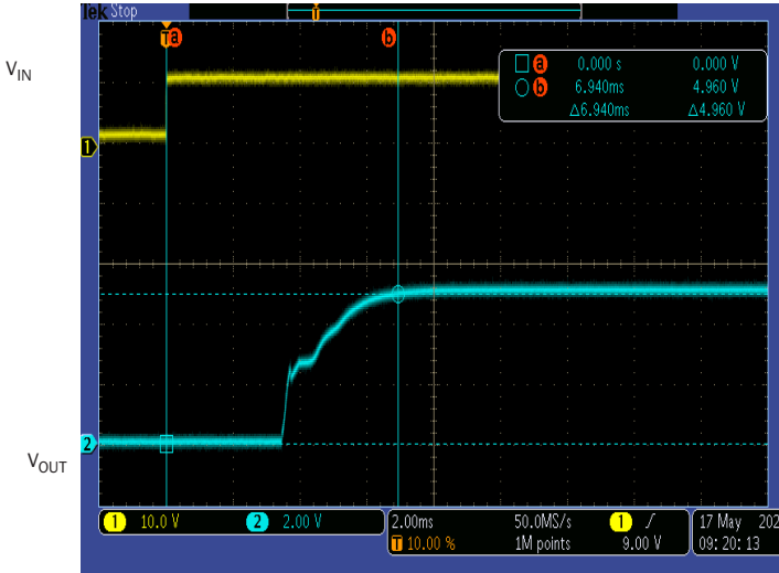
MSA+2805S START-UP RESPONSE FULL LOAD W 500uF CAP FIGURE 20
