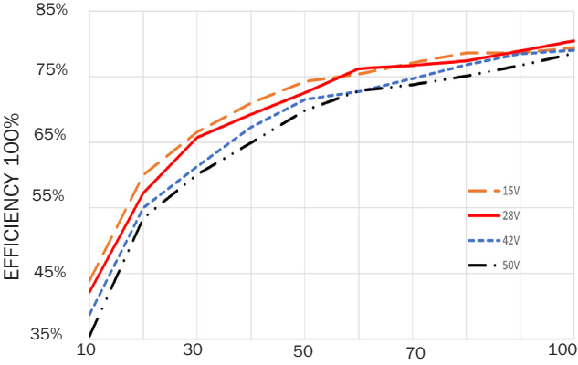
OUTPUT POWER MSA+2815S EFFICIENCY FIGURE 11
