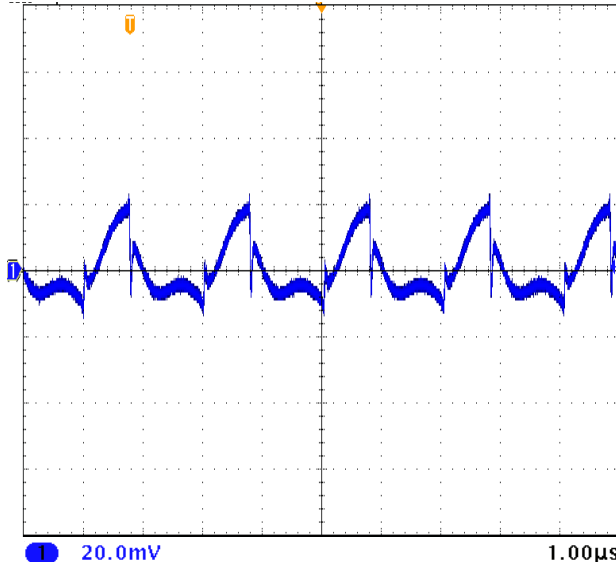
BW 20 Hz - 20 MHz UNITS ARE PER DIVISION MFX2805S OUTPUT RIPPLE FIGURE 19
