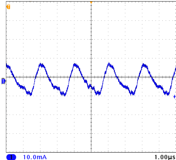
BW 20 Hz - 20 MHz UNITS ARE PER DIVISION MFX2805S INPUT RIPPLE FIGURE 18
