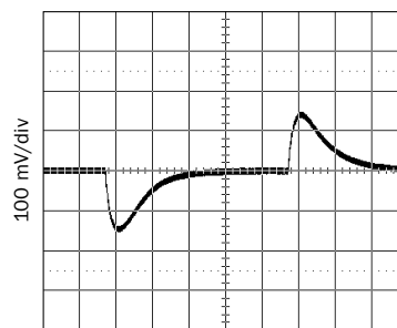
MFP0507S Load Transient FIGURE 16
