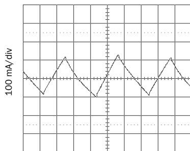
MFP0507S Input Ripple (I IN ) FIGURE 12
