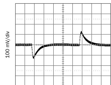
MFP0507S Load Transient FIGURE 17
