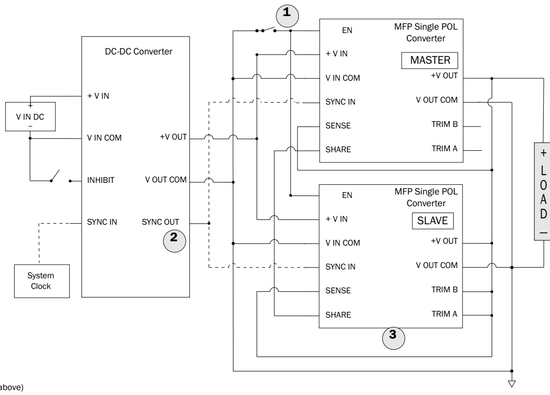
FIGURE 9: TYPICAL SHARE CONNECTION WITH OPTIONAL SYNC
