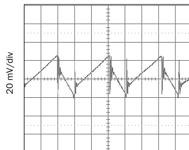
MFP0507S Output Ripple FIGURE 15
