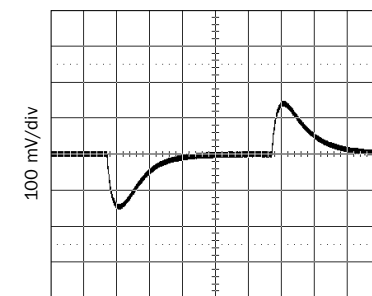
200 μs/div 3.3 V IN , 1.2 V OUT , 5 A load MFP0507S Load Transient FIGURE 16
