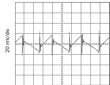
1 μs/div 3.3 V IN , 1.2 V OUT , 5 A load MFP0507S Output Ripple FIGURE 14
