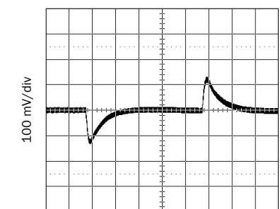
200 μs/div 5 V IN , 3.3 V OUT , 5 A load MFP0507S Load Transient FIGURE 17
