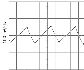
1 μs/div 5 V IN , 3.3 V OUT , 5 A load MFP0507S Input Ripple (I IN ) FIGURE 13
