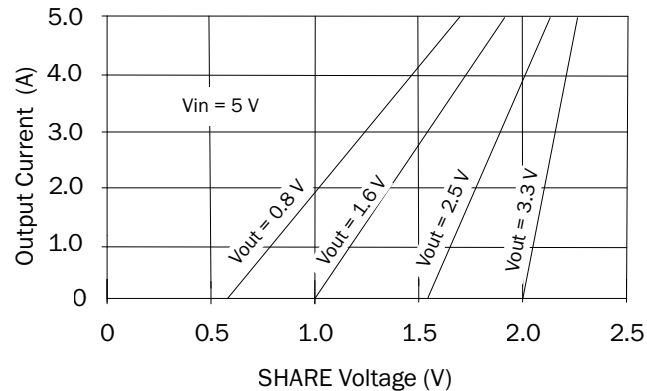
FIGURE 18: SHARE AS MONITOR FOR OUTPUT CURRENT
