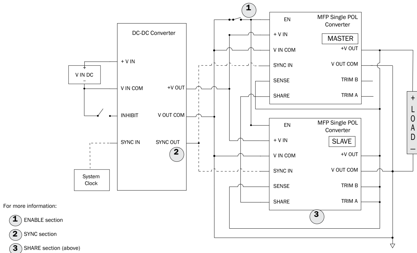
FIGURE 9: TYPICAL SHARE CONNECTION WITH OPTIONAL SYNC
