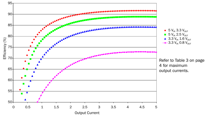
FIGURE 11: TYPICAL EFFICIENCIES
