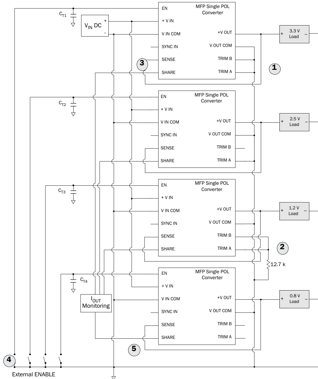
FIGURE 5: TYPICAL CONNECTION DIAGRAM ENABLE, TRIM, SENSE, AND I_{OUT} MONITORING
