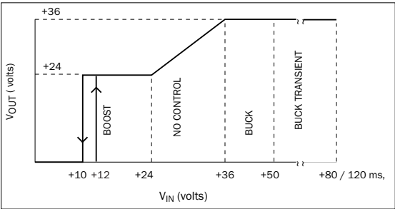
FIGURE 2: OUTPUT VOLTAGE
