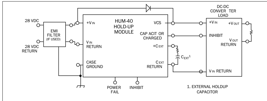
FIGURE 1: HUM-40 MODULE SYSTEM BLOCK DIAGRAM
