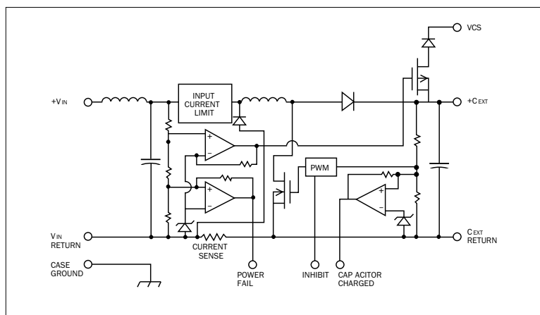
FIGURE 2: HUM-40 MODULE BLOCK DIAGRAM
