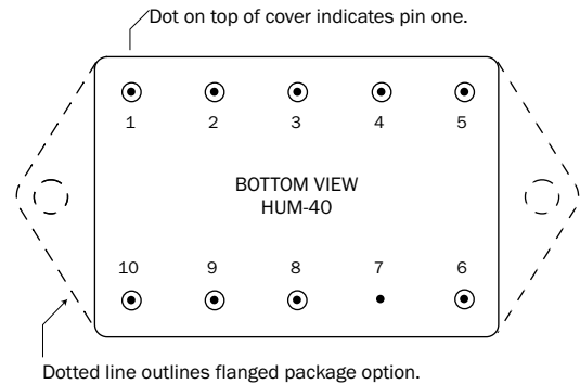
FIGURE 4: PIN OUT FLANGED AND NON-FLANGED
