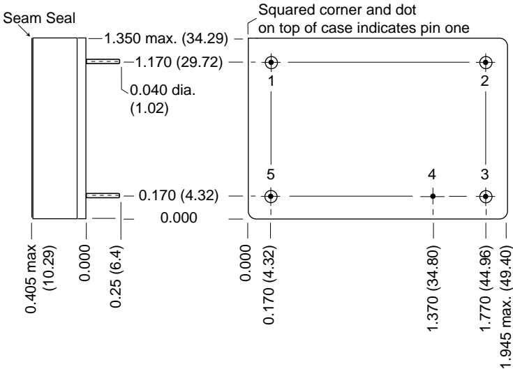
BOTTOM VIEW CASE F5
