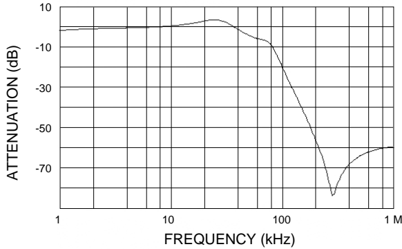
FMCE-0828 Attenuation
