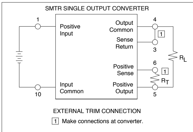
FIGURE 1: TRIM CONNECTION 1, 2, 3, 4
