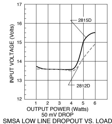
SMSA LOW LINE DROPOUT VS. LOAD
