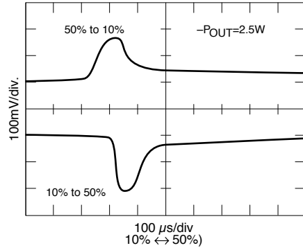
SMSA2815D +V O STEP LOAD RESPONSE
