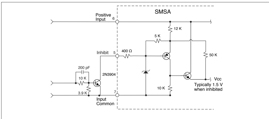
FIGURE 2: INHIBIT INTERFACE
