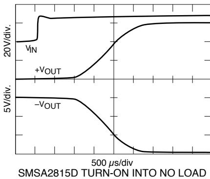
SMSA2815D TURN-ON INTO NO LOAD
