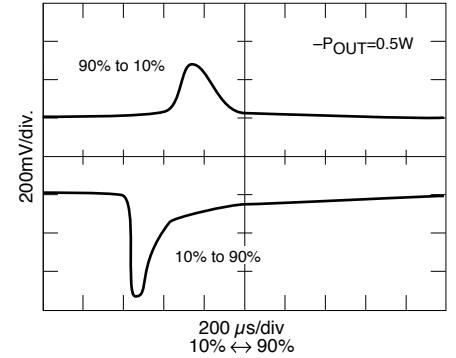
SMSA2815D +V O STEP LOAD RESPONSE
