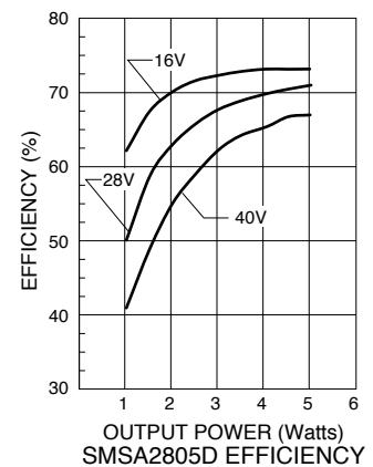
SMSA2805D EFFICIENCY
