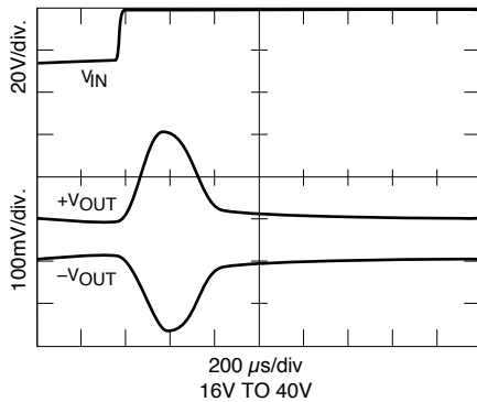
SMSA2815D INPUT STEP LINE RESPONSE
