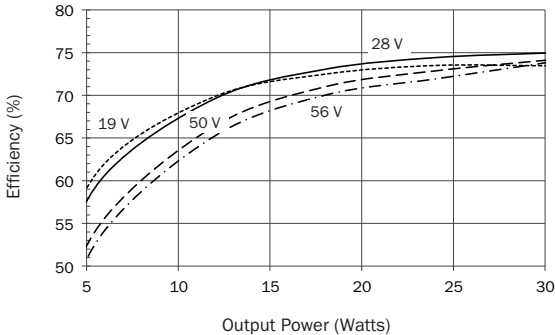
SMRT28512T Efficiency
