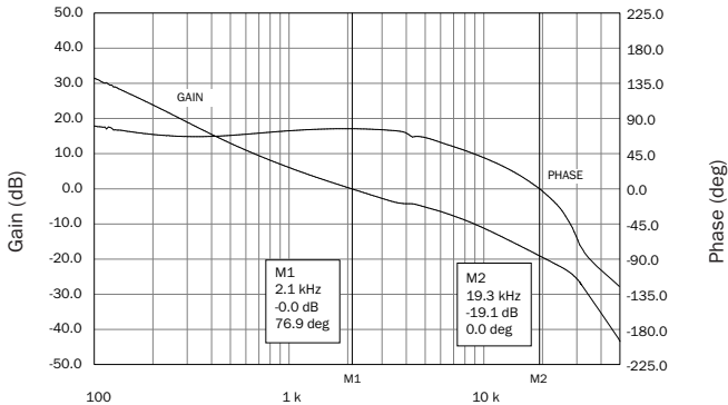
SMRT28507T Gain Phase, +Aux
