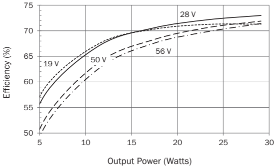
SMRT28507T Efficiency
