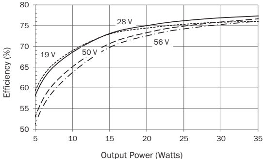
SMRT2812D Efficiency FIGURE 29
