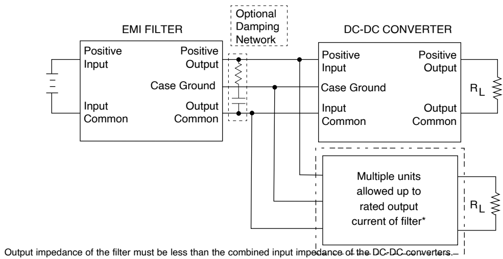
FIGURE 2: Connection Diagram
