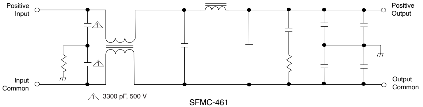
FIGURE 1: SFMC28-461 Schematic
