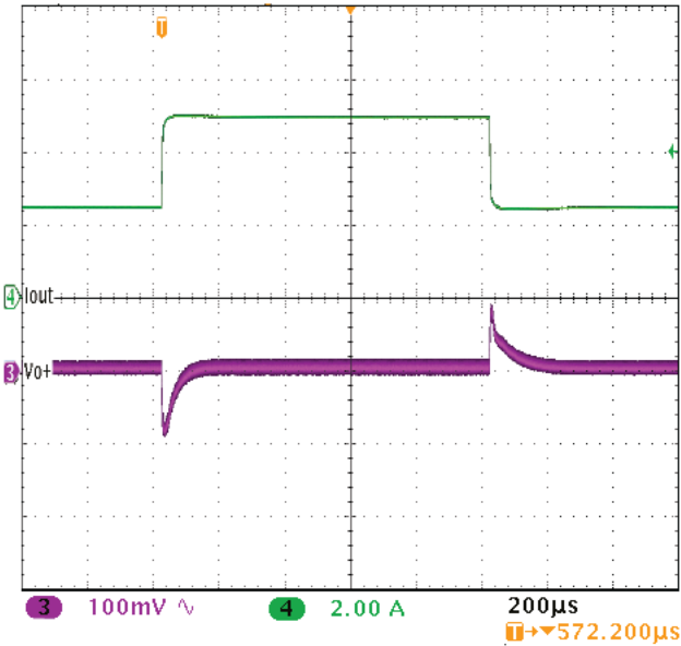
UNITS ARE PER DIVISION MTR2805S STEP LOAD 50% - 100% - 50%
