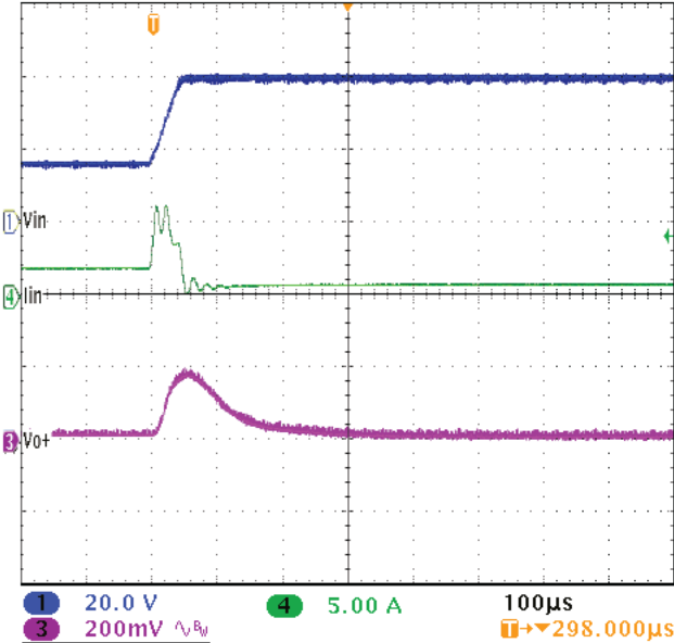
UNITS ARE PER DIVISION MTR2805S STEP LINE 16 - 40 VOLTS
