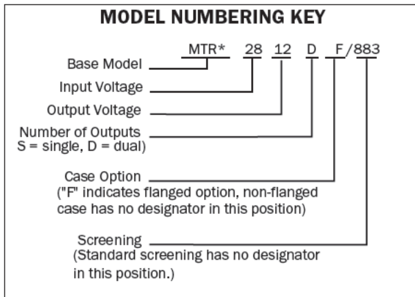
FIGURE 7: MTR (50) MODEL NUMBERING KEY
