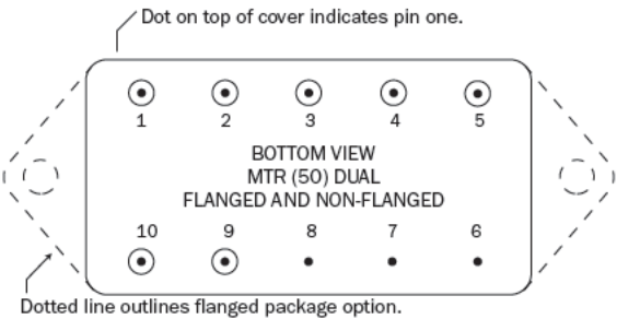
FIGURE 6: MTR (50) PIN OUT DUAL OUTPUT MODELS
