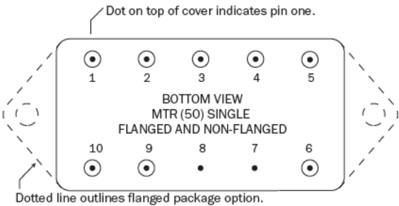
FIGURE 5: MTR (50) PIN OUT SINGLE OUTPUT MODELS
