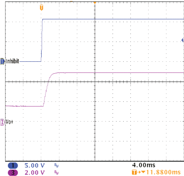
5 VOLT SINGLE - START-UP INTO NO LOAD
