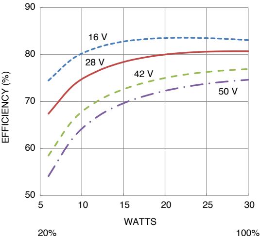
MTR2812S EFFICIENCY FIGURE 12
