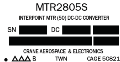
FIGURE 8: COVER MARKING FOR MTR (50) - 50 VIN
