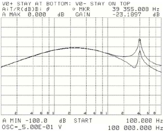
AUDIO REJECTION - 28 VIN REPRESENTATIVE OF DUAL OUTPUTS
