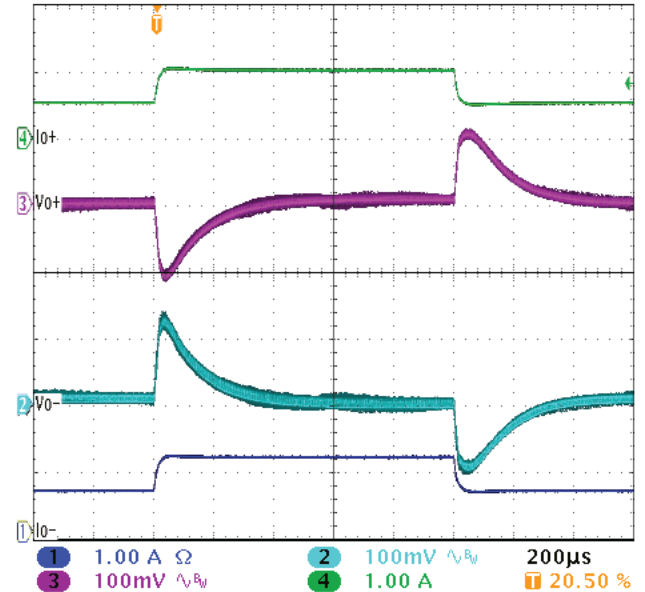
UNITS ARE PER DIVISION MTR2815D STEP LOAD 50% - 100% - 50% FIGURE 25
