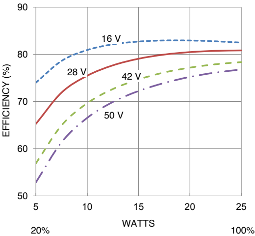
MTR288R5S EFFICIENCY FIGURE 11
