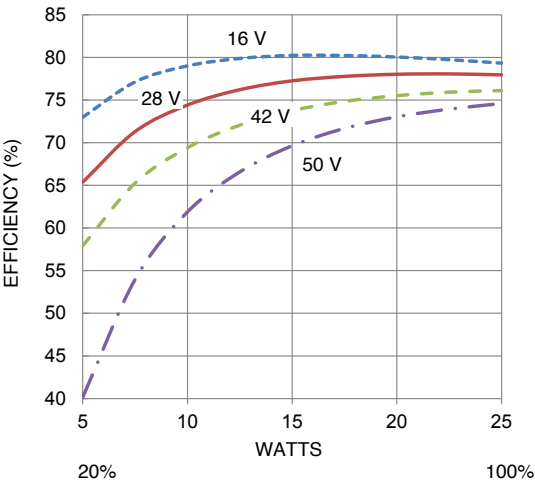
MTR2805S EFFICIENCY FIGURE 10
