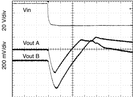
100 \mu s/div Vin 56 to 19 V, full resistive load
