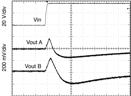
100 \mu s/div Vin 19 to 56 V, full resistive load
