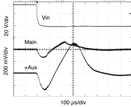
V_{in} 56 to 19 V, full resistive load SMRT283R312T Representative of Triple Output Line Transient FIGURE 48
