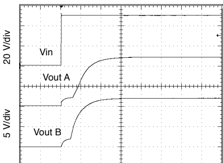
4 ms/div Full resistive load, 50 Vin
