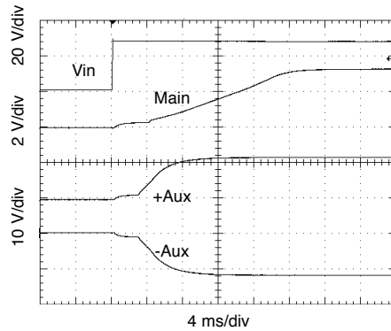
Full resistive load, 28 V_{in} SMRT283R312T Representative of Triple Output Turn On Delay FIGURE 51
