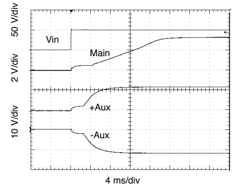
Full resistive load, 50 V_{in} SMRT283R312T Representative of Triple Output Turn On Delay FIGURE 52
