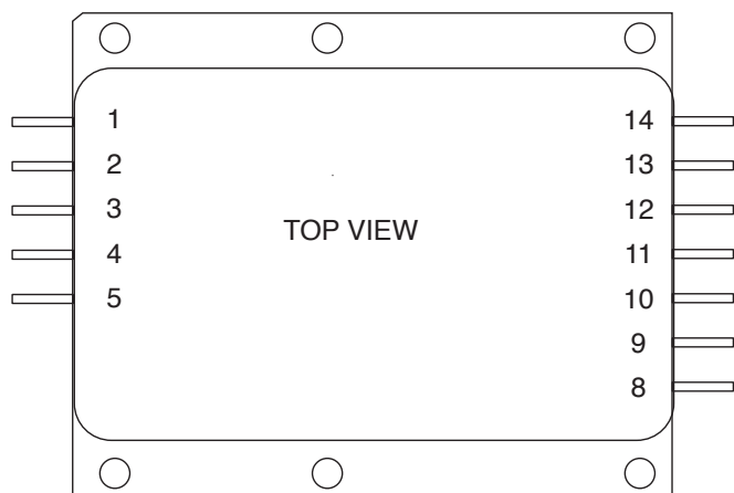
FIGURE 6: PIN OUT
