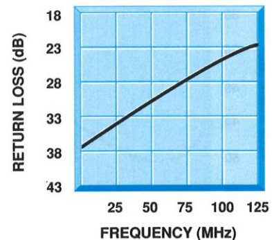
RETURN LOSS vs. FREQUENCY
