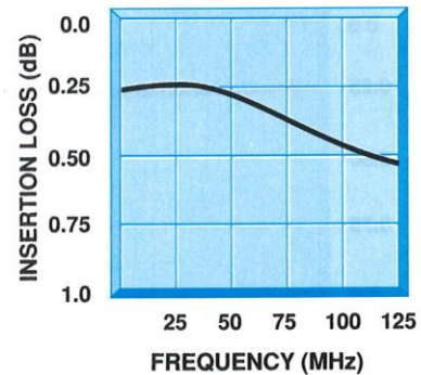
INSERTION LOSS vs. FREQUENCY
