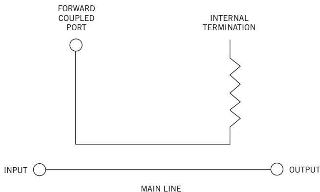
Figure 1: Three Port Directional Coupler
