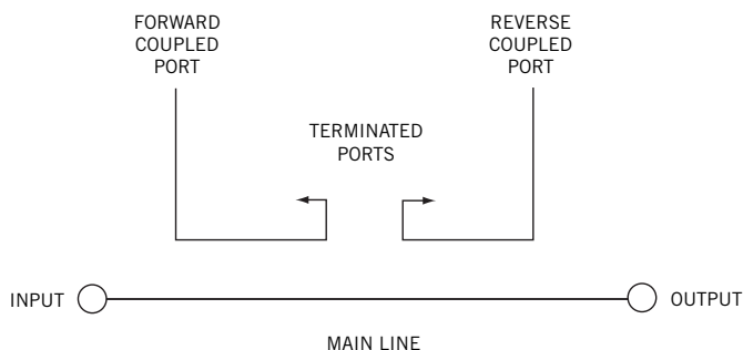
Figure 4: Four Port Dual Directional Coupler
