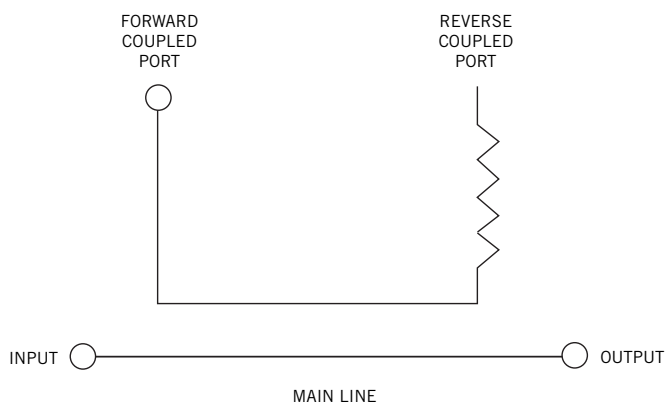
Figure 3: Four Port Bi-Directional Coupler
